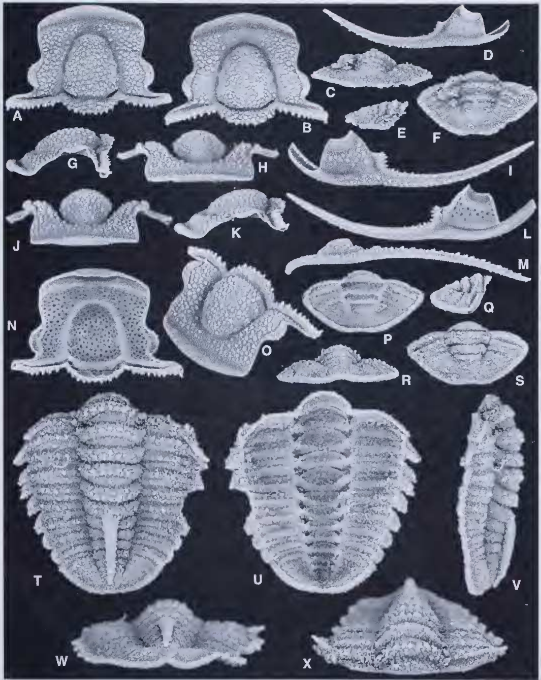
FIG. 6. Hinzecurus paragenalatus (Ross, 1951). A-S from the Garden City Formation (Skullrockian, Bellefontia-Xenostegium Zone), Franklin Basin, section FB7 39.0-44.2m; topotype material. A, G, J, N, O, cranidium, SUI 99569, dorsal, left lateral, anterior, ventral and oblique views, \times 6 . B, H, K, cranidium, SUI 99570, dorsal, anterior and left lateral views, \times 6 . C, E, F, pygidium, SUI 99571, posterior, right lateral and dorsal views, \times 7.5 . D, right librigena, SUI 99572, external view, \times 6 . I, L, M, left librigena, SUI 99573, external, internal and ventrolateral views, \times 6 . P-S, pygidium, SUI 99574, ventral, right lateral, posterior and dorsal views, \times 7.5 . T-X from the Red Canyon Member, House Formation (Skullrockian, Bellefontia-Xenostegium Zone), Ibex area, section Lava Dam North 144.0m, thoracopygidium, SUI 99751, dorsal, ventral, left lateral, posterior and anterior views, \times 7.5 .
